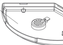
JBL CP i60-200 greenline base plate with valve
