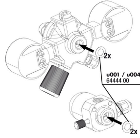
JBL ProFlora "u" o-ring conta 2x
