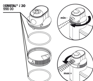
JBL PC i30 water outlet with regulation
