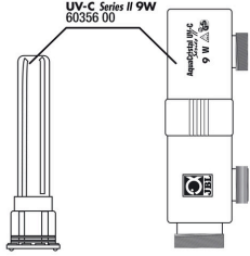
JBL AC UV-C II 9 W gövde+cam
