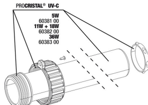
JBL PC UV-C quartz glass cylinder set
